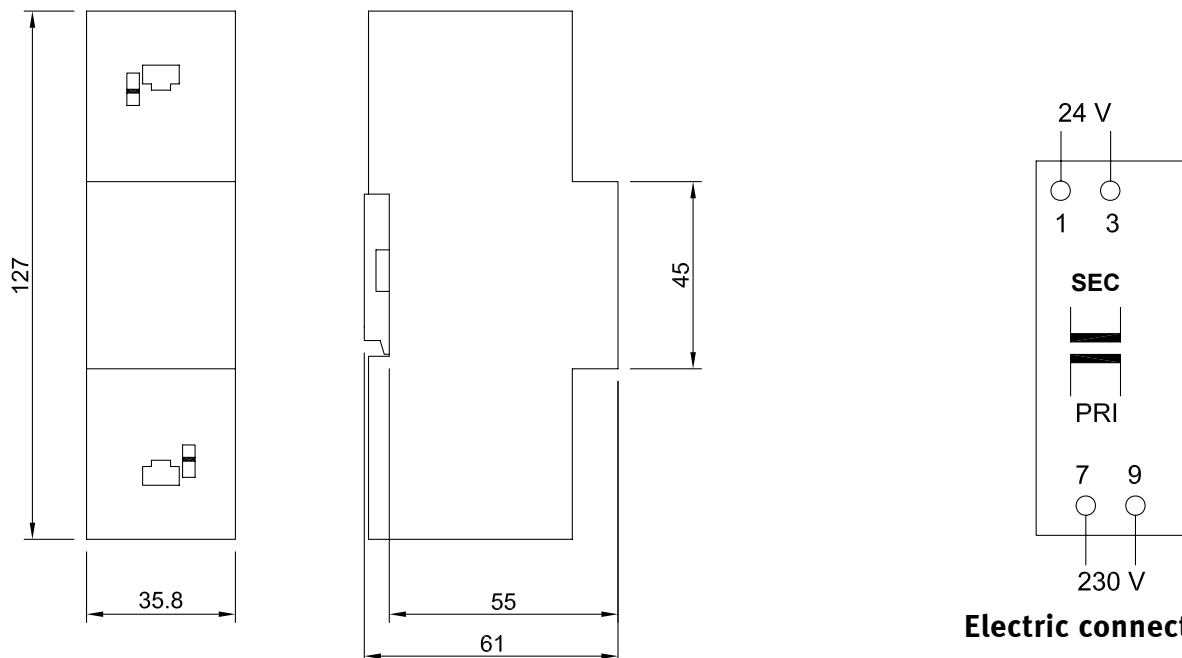
Dimensional drawing
